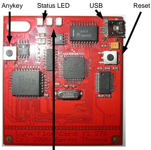
USB-Transfer LEDs (rot=upload, grün=download)
