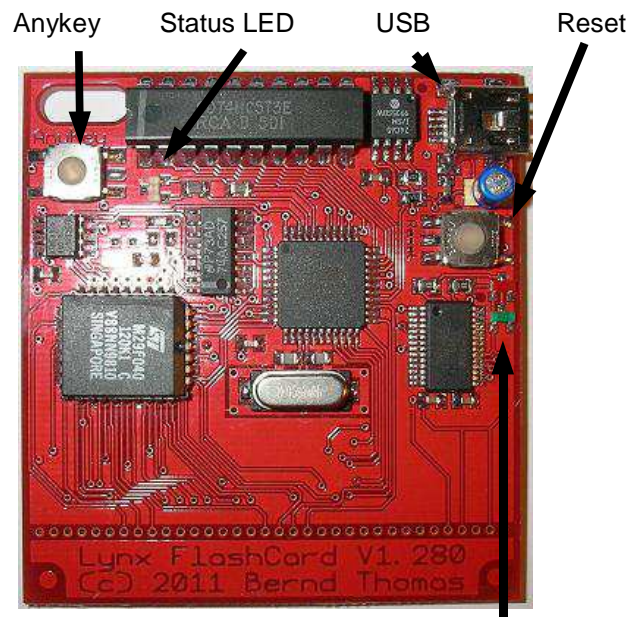
USB-Transfer LEDs (rot=upload, grün=download)
